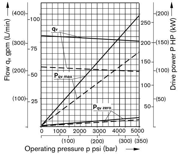
Size 180
