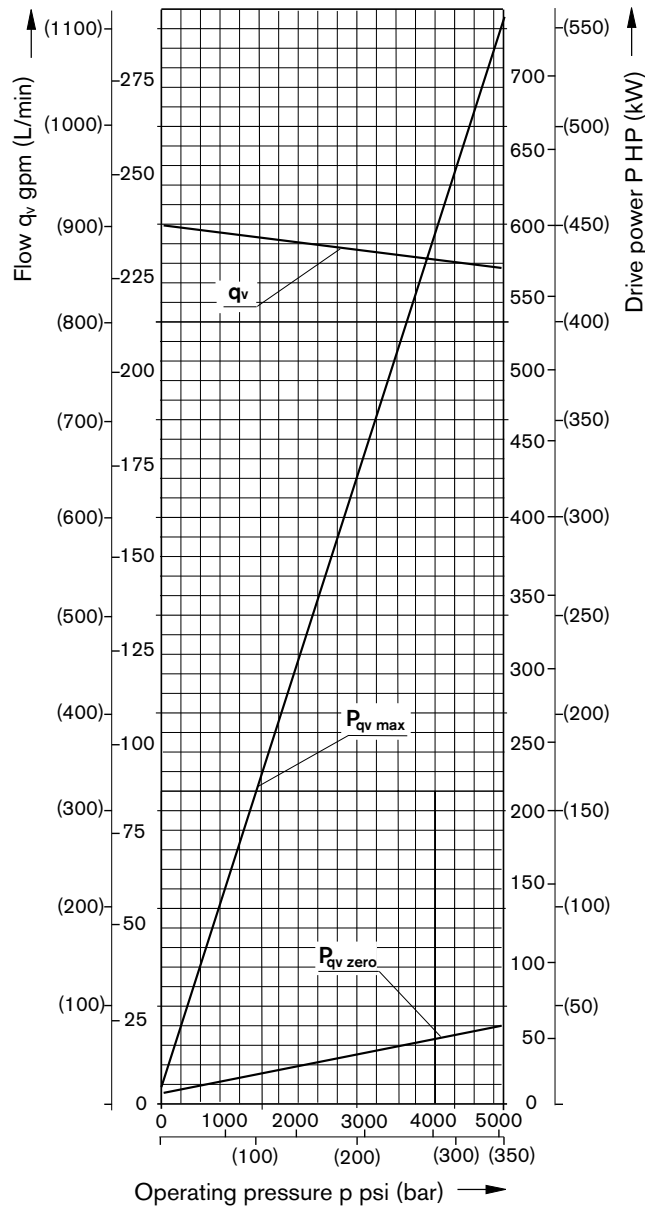
Size 750
