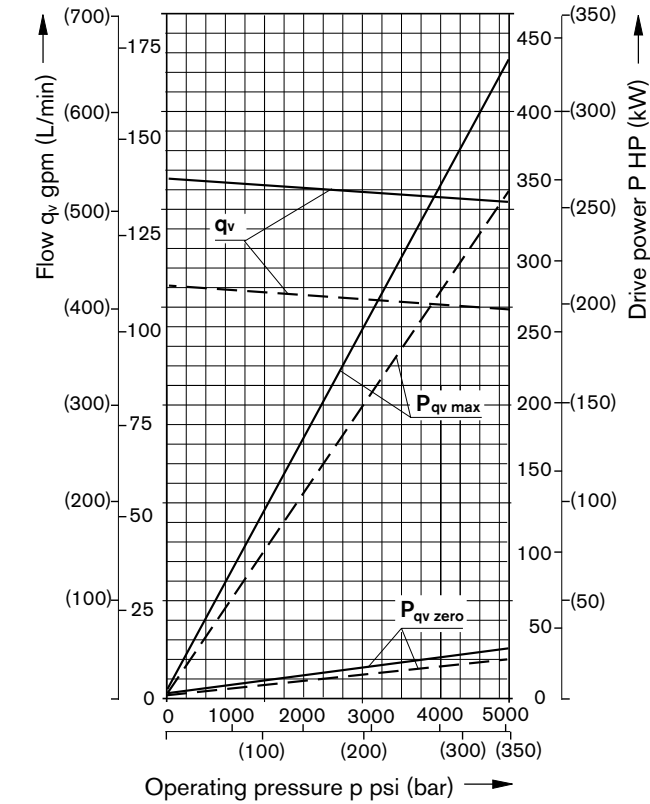
Size 355
