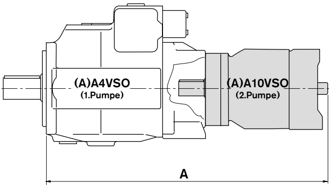
(A)A4VSO + (A)A10VSO
