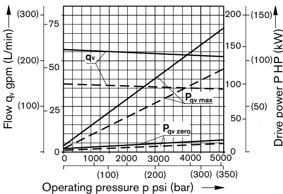
Size 125
