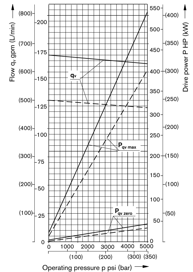
Size 500
