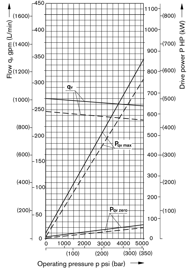
Size 1000
