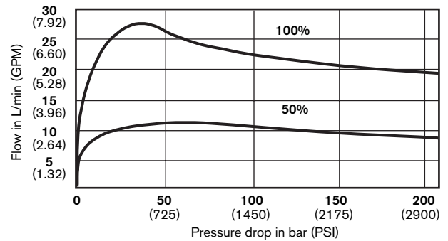
4WRAB6E25-1X
