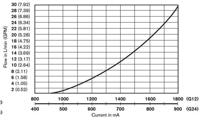
4WRAB6E25-1X
