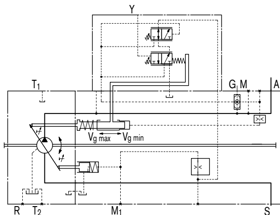
Size 190 to 260
