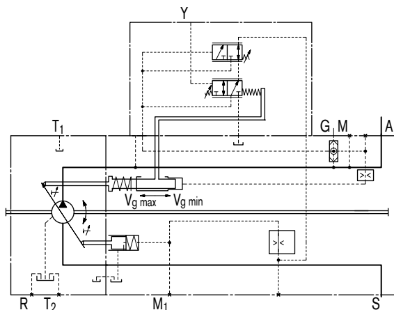
Size 190 to 260
