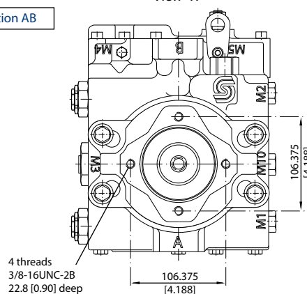
View "X"
