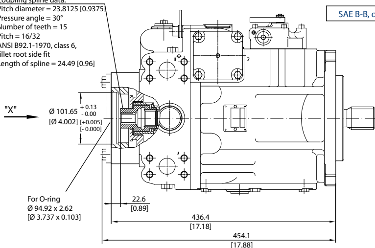
Shaft dimensions
